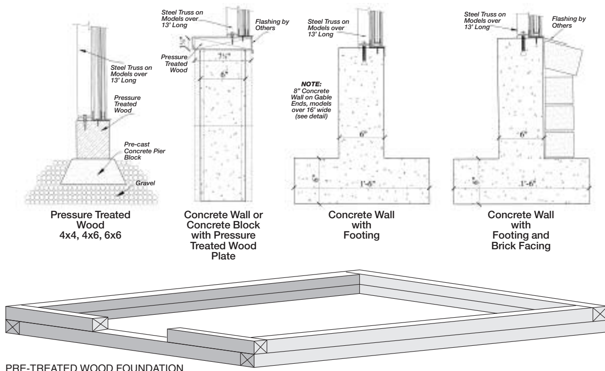
PRE-TREATED WOOD FOUNDATION
